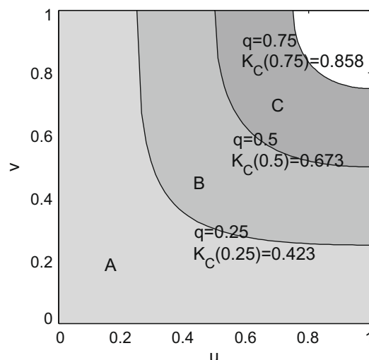
Fig. 1. Distribution function K_C of Gumbel-Hougaard Archimedean copulas with dependence parameter \theta = 2 . K_C provides the probability measure for the shaded region where C(u, v) \leq q ( K_C(0.25) for region A, K_C(0.5) for regions A + B, and K_C(0.75) for regions A + B + C).
