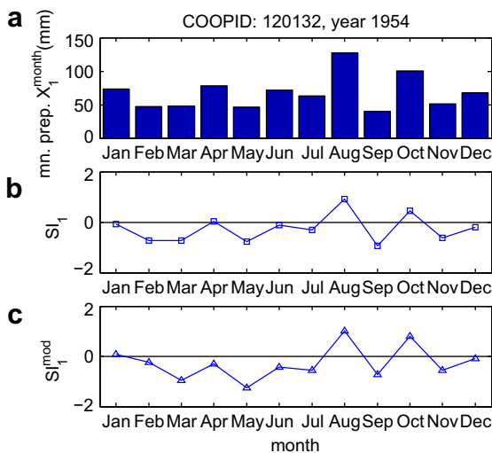
Fig. 4. Comparison between conventional and modified 1-month SI using precipitation station Alpine 2 NE (COOPID: 120132): (a) upper panel: monthly precipitation of year 1954 ( X_1^{\text{month}} series); (b) middle panel: conventional SI_1 of each month; (c) lower panel: modified SI_1^{\text{mod}} of each month.
