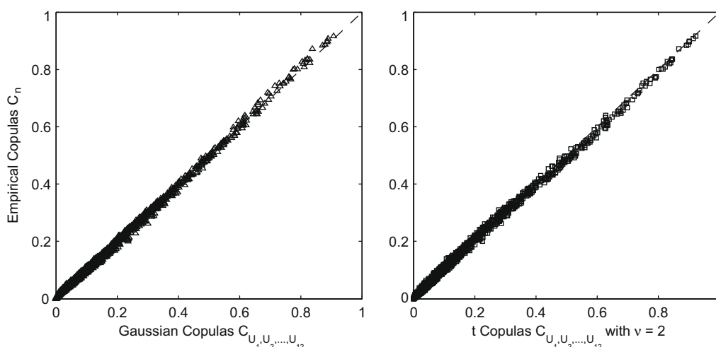
Fig. A.1. Empirical copulas C_n (Eq. (2)) versus (a) left: Gaussian (Eq. (A.1) with \nu \rightarrow \infty ) and (b) right: Student t -copulas (Eq. (A.1) with \nu = 2 ) for precipitation marginals \{u_1^{\text{mod}}, u_2^{\text{mod}}, \dots, u_{12}^{\text{mod}}\} of station Alpine 2 NE (COOPID: 120132). The dash line corresponds to the 45-degree line.
