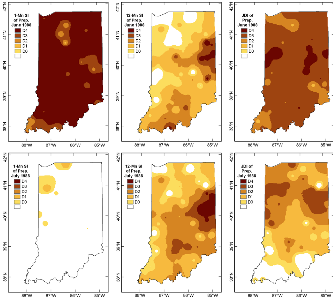
Fig. 6. Regional illustration of SI_1^{mod} (left), SI_{12}^{mod} (middle), and JDI (right) of precipitation of Indiana for June and July 1988.
