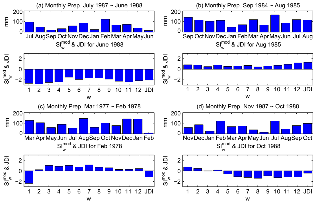
Fig. 5. Illustration of JDI and SI_w^{mod} , w = 1, 2, \dots, 12 of precipitation station Alpine 2 NE (COOPID: 120132) for four selected cases.
