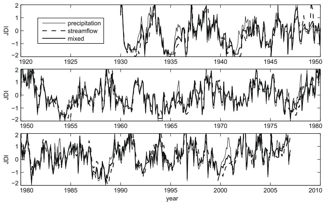
Fig. 7. Comparison of various JDIs constructed by precipitation marginals \{u_1^{\text{mod}}, u_2^{\text{mod}}, \dots, u_{12}^{\text{mod}}\} of station Alpine 2 NE (COOPID: 120132), streamflow marginals \{v_1^{\text{mod}}, v_2^{\text{mod}}, \dots, v_{12}^{\text{mod}}\} of station Whitewater River (USGS Site 03275000), and mixed marginals \{u_1^{\text{mod}}, \dots, u_{12}^{\text{mod}}, v_1^{\text{mod}}, \dots, v_{12}^{\text{mod}}\} .
